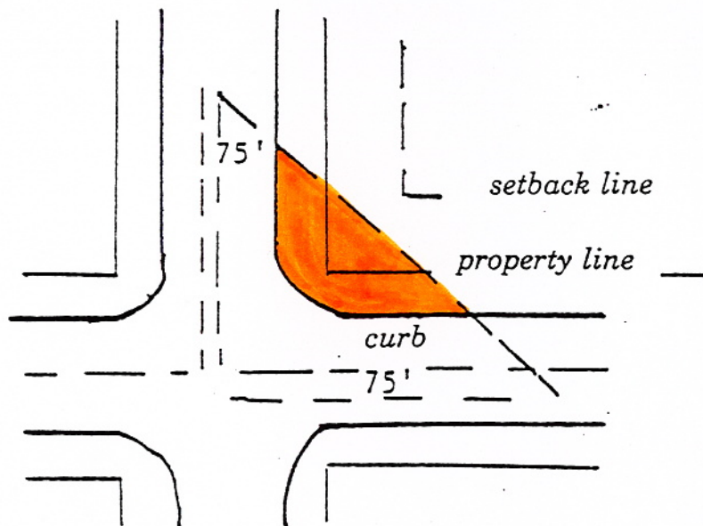
Sight Triangle Illustration Minimum Standard
